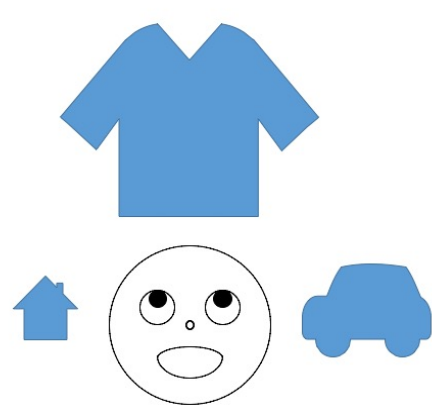
Incongruent
