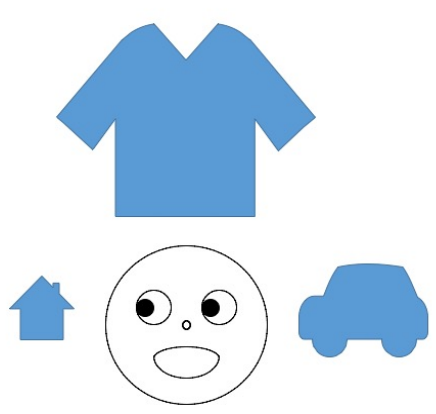
Congruent
