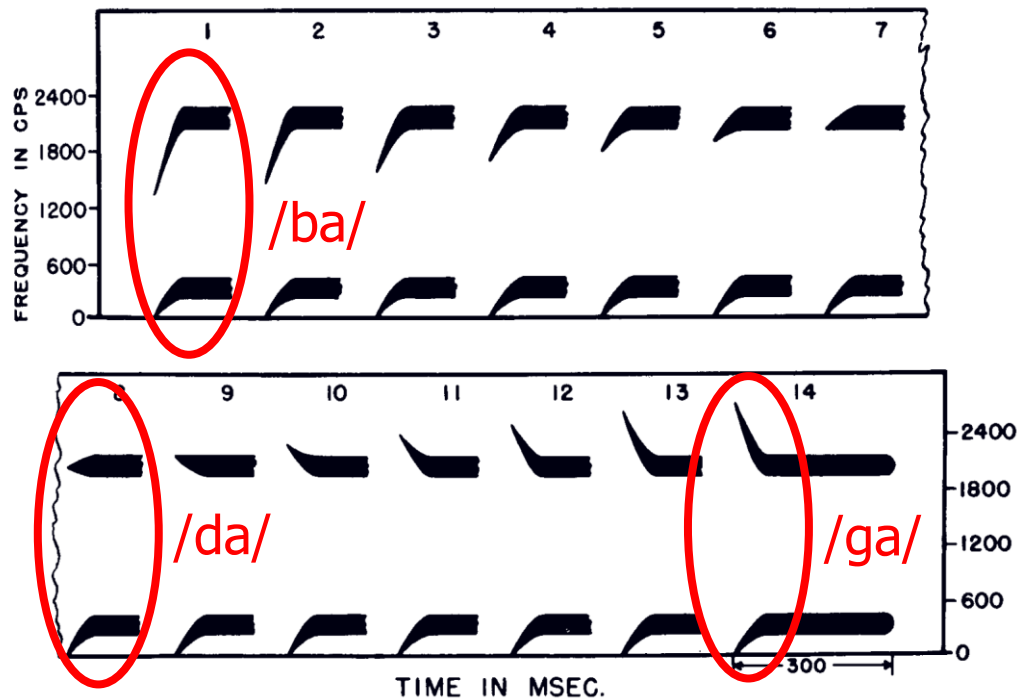
Figure 5.23. Two-formant synthetic CV pattern series: the stimuli for /ba/, /da/, and /ga/. (Reprinted with permission from A. M. Liberman et al. : Journal of Experimental Psychology . 54, © 1957, American Psychological Association.)
