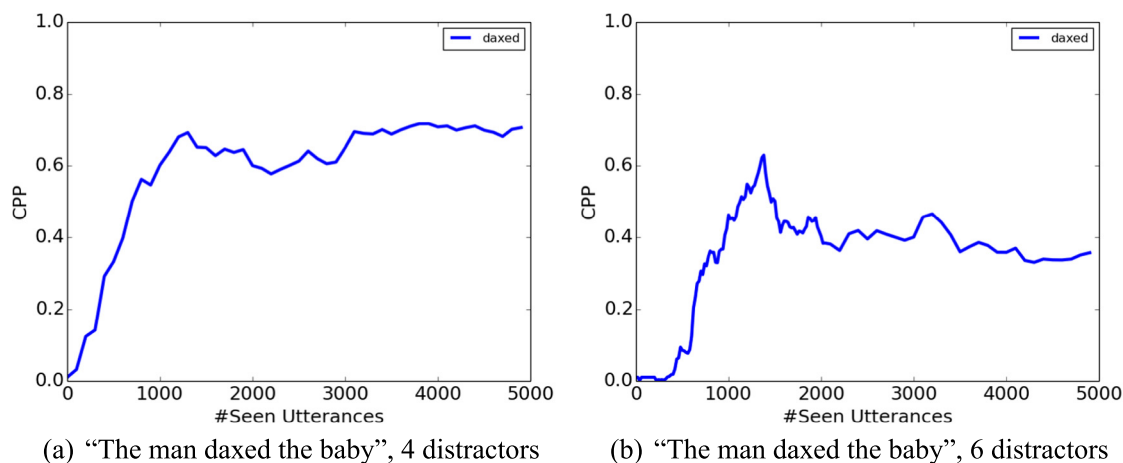
Fig. 15. Syntactic bootstrapping: The model's CPP for the unknown word “daxed” ( y -axis) after training on n utterances from the corpus ( x -axis) followed by a single presentation of the sentence “The man daxed the baby” with SVO/OVS ambiguous semantics. During training only, either four (a) or six (b) distractors are included along with each correct logical form.
