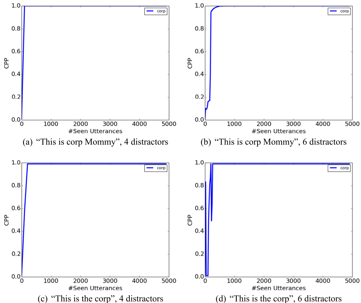
Fig. 17. The correct production probability (y-axis) for the unknown word “corp” in the sentences “This is corp Mommy”, where it should be interpreted as a preposition (a and b), and “This is the corp” (c and d), where it should be interpreted as a noun, as a function of the number of training examples seen (x-axis). The model is trained in the 4 and 6 distractors settings.
