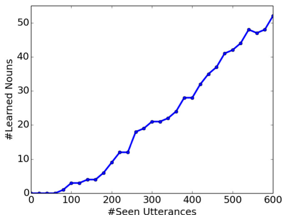
Fig. 12. The size of the production vocabulary of nouns as a function of the number of utterances seen, for the 6 distractors setting. The production vocabulary is defined as all nouns with a CPP of at least 0.8.
