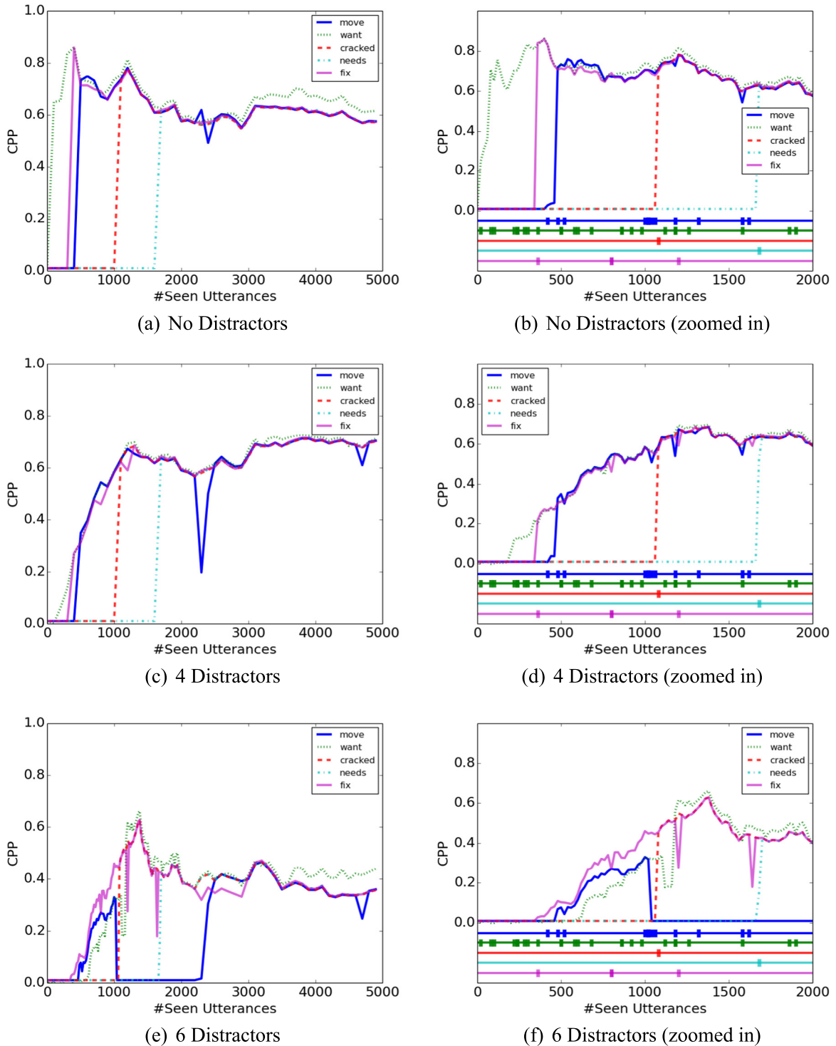
Fig. 7. Learning curves showing the correct production probability for verbs of different frequencies in the (top) 0-distractor, (middle) 4-distractor, and (bottom) 6-distractor settings, as a function of the number of utterances observed. (Results from the 2 distractor setting in this case are uninformative since the model fails to learn SVO word order well: see Fig. 3(b) and associated discussion.) Plots on the right zoom in on the first stage of learning, and also show horizontal “timelines” for each word with tickmarks indicating, for each 20-utterance block, whether the word occurred in that block. (The color and top-to-bottom order of the timelines matches the words in the legend.) Large jumps in the plots generally correspond to observations in which the given verb appears, while smaller changes can occur due to fine-tuning of higher-order model parameters (e.g., the overall probability of transitive verbs having SVO syntax). The frequencies for these verbs are: f(\text{move}) = 3 , f(\text{want}) = 70 , f(\text{cracked}) = 1 , f(\text{needs}) = 3 , f(\text{fix}) = 11 .
