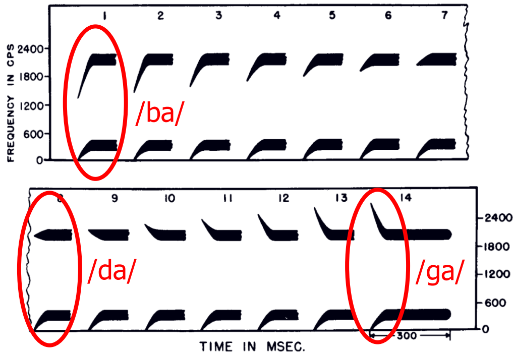
Figure 5.23. Two-formant synthetic CV pattern series: the stimuli for /ba/, /da/, and /ga/. (Reprinted with permission from A. M. Liberman et al.: Journal of Experimental Psychology . 54, © 1957, American Psychological Association.)
