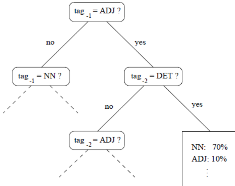
Figure 1: A sample decision tree
