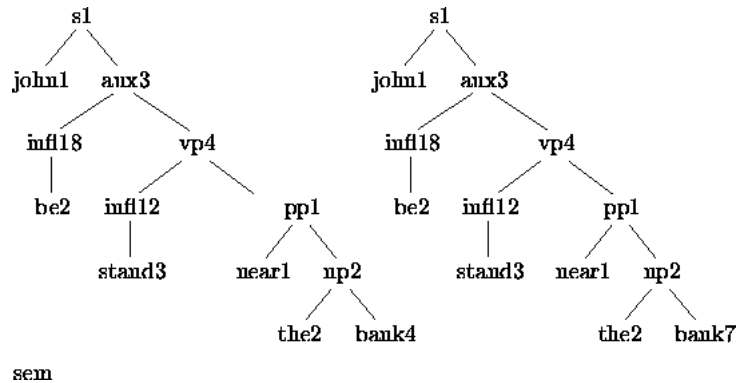
Figure 5.6: Derivation trees
