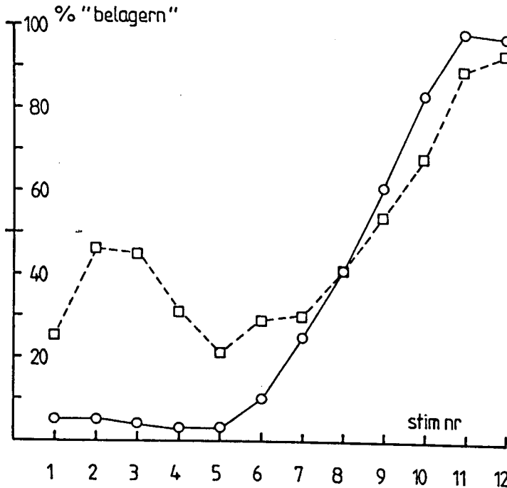
Fig. 3. Percentage stem-stress responses for "umlagern" (= "belagern") in the series of 12 F0 peak positions combined with the original prefix-stress utterance of "Er wird's wohl umlagern."; original, sharply falling peak contour (continuous line, at each data point N=14 \times 10 + 9 \times 5 = 185 ), and slowly falling peak contour, transferred from the original stem-stress utterance (broken line, at each data point N=16 \times 5 = 80 ).
