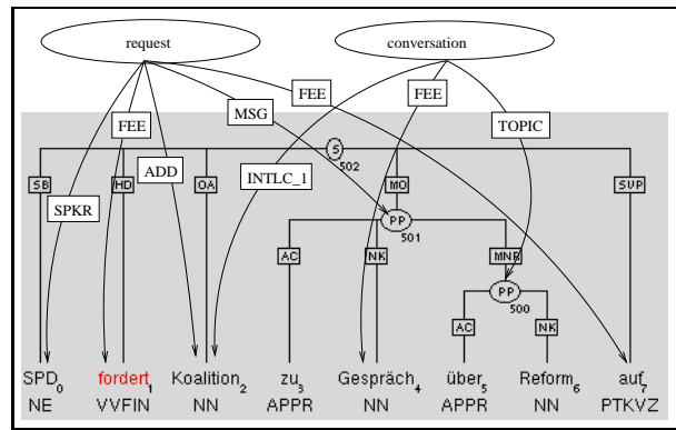
Figure 3: Frame annotation.
