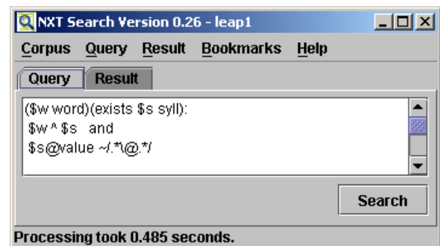
Figure 3: NXT Search
