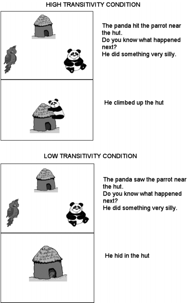
Figure 1. Example stimuli for high and low transitivity conditions.
