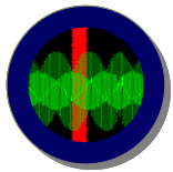
sound waves
