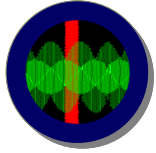
sound waves
